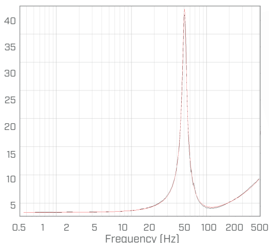
Magnitude of electric impedance
